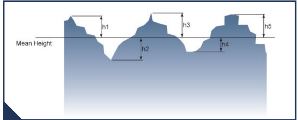
Figure 2 - surface roughness
